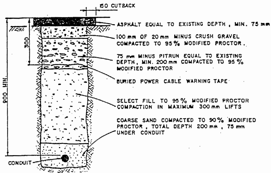
TYPICAL TRENCH IN ROAD STRUCTURE
