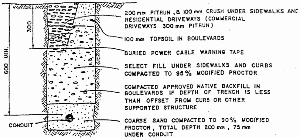
TYPICAL TRENCH
